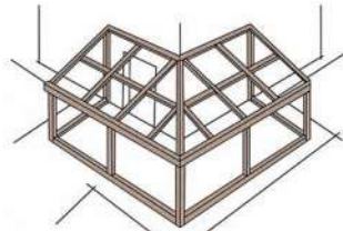
Gazebo in the External Corner of the House
